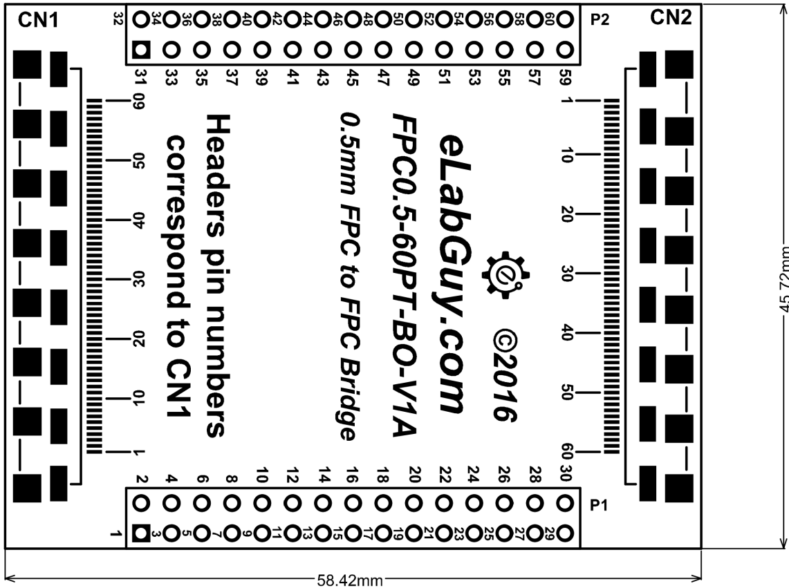
PCB outline Drawing
